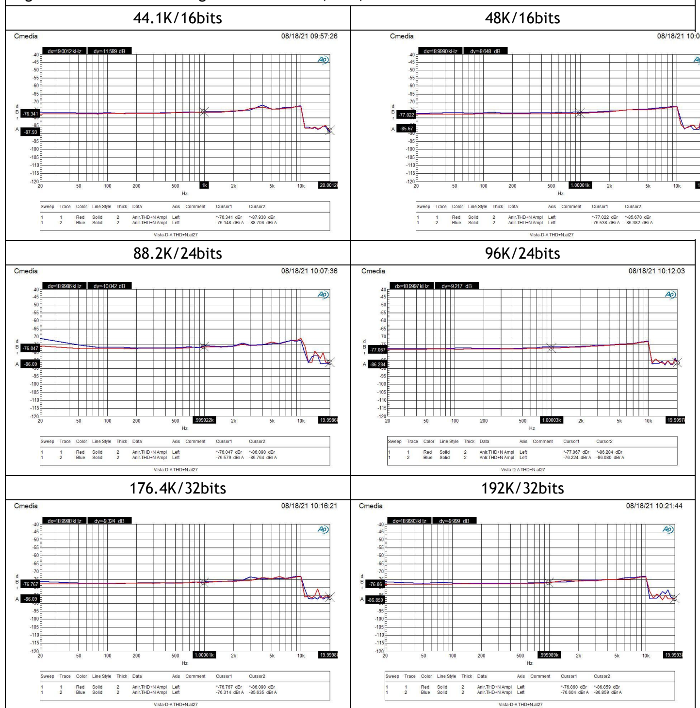
Figure 5 : DAC 32Ω loading Cascade 33 ohm, 0dB, THD+N
