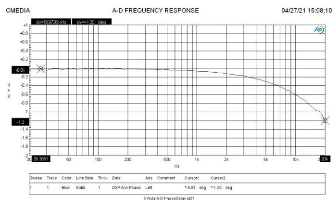
Figure 23 : ADC Interchannel phase delay 0dB Gain
