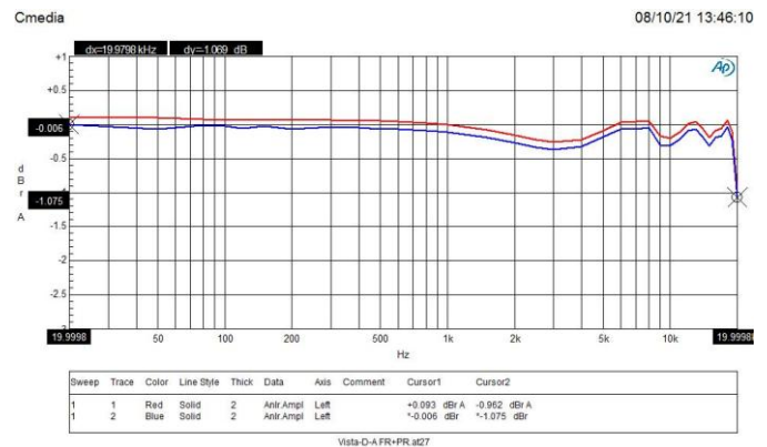
Figure 12 : DAC 32Ω loading Cascade 33 Ω ,Frequency Response
