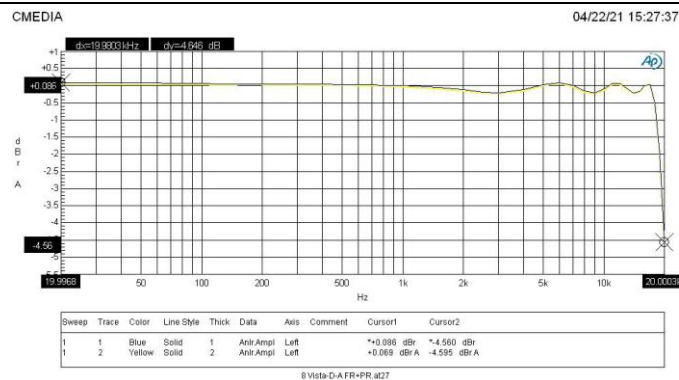
Figure 11 : DAC 32Ω loading, Frequency Response
