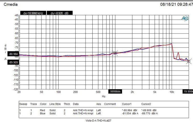
Figure 4 : DAC 32Ω loading, -3dB, THD+N
