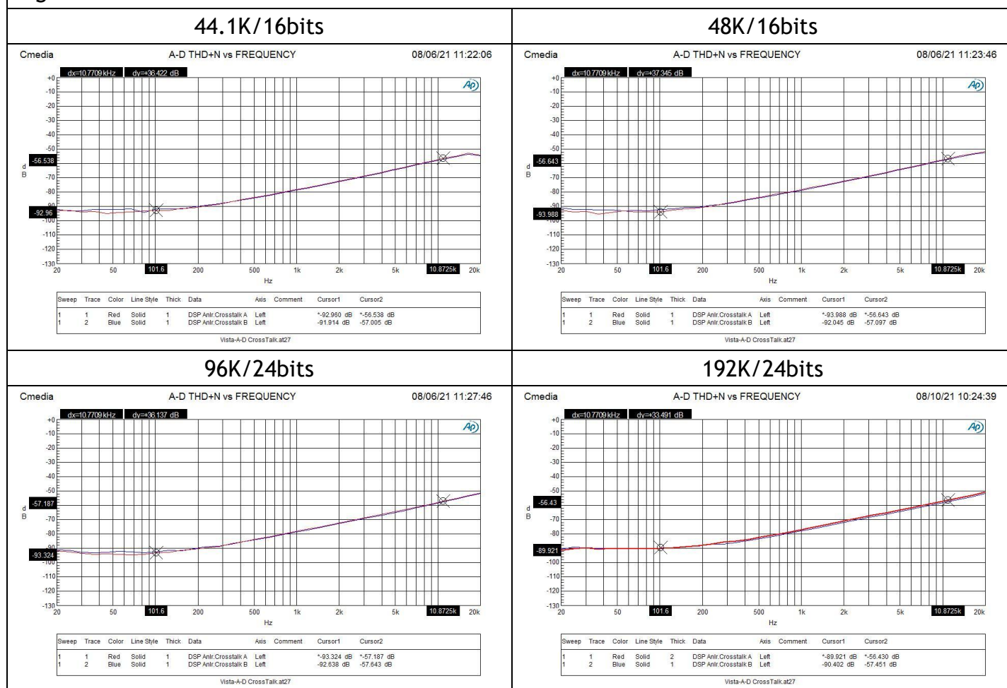
Figure 20 : ADC Cross-talk 20dB Gain
