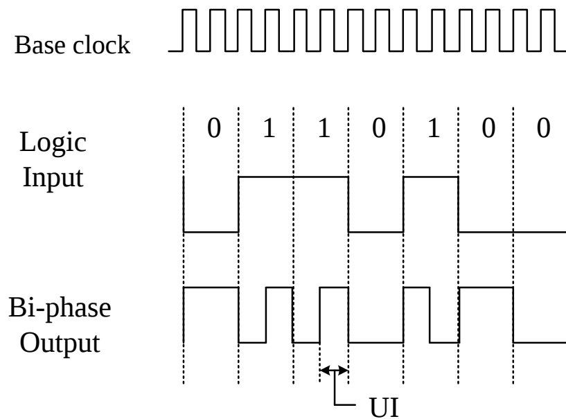
Fig. 6.3.2 S/PDIF biphasemark-code (BMC).
