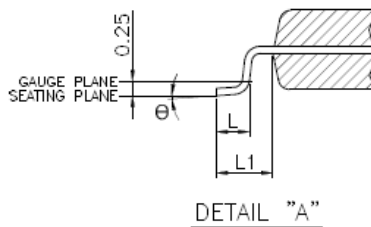
Package Dimension of CM6535
