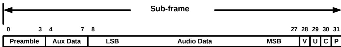
Figure -5 SPDIF Subframe Description
