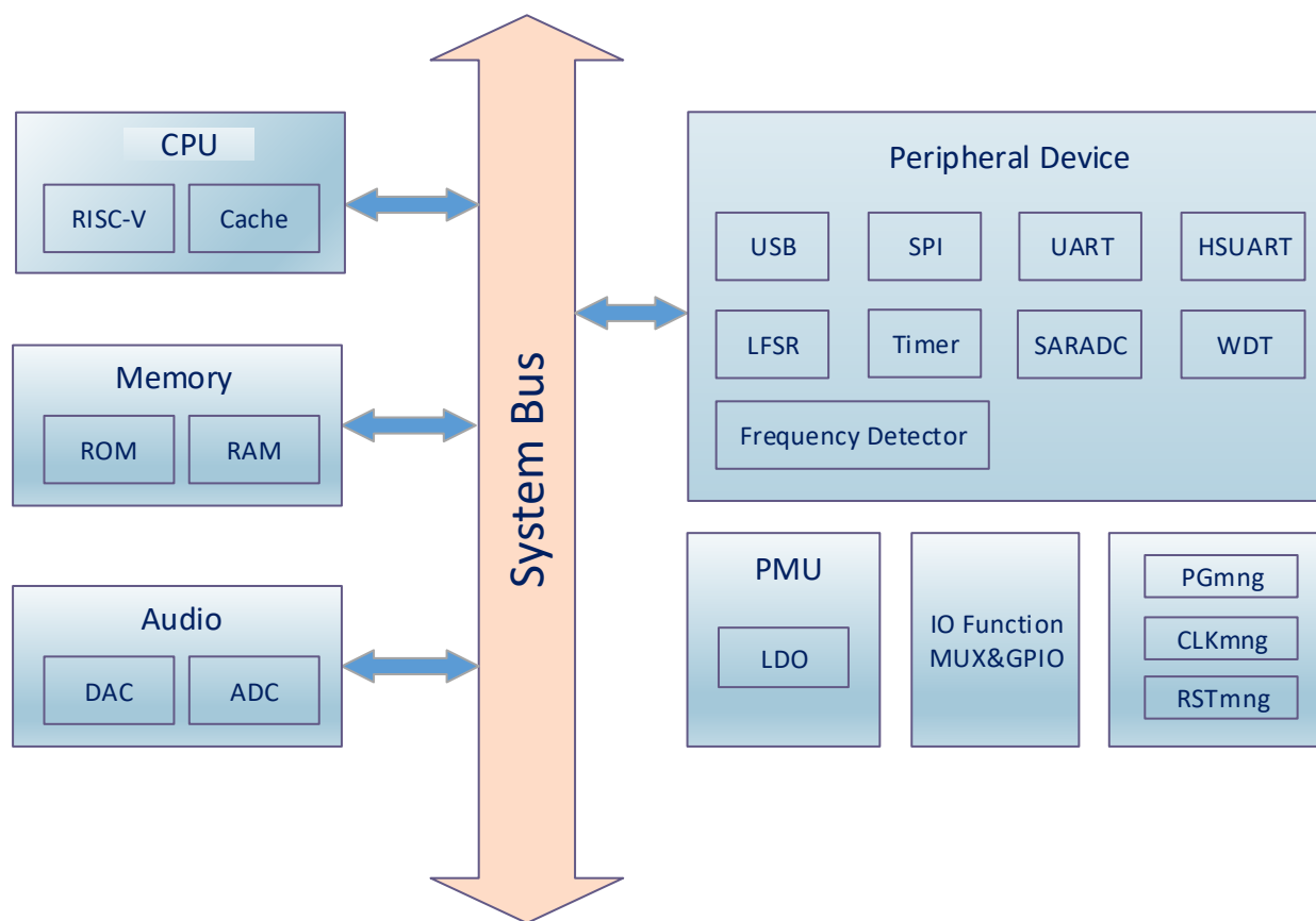
Figure 2-1 Architecture Block Diagram
