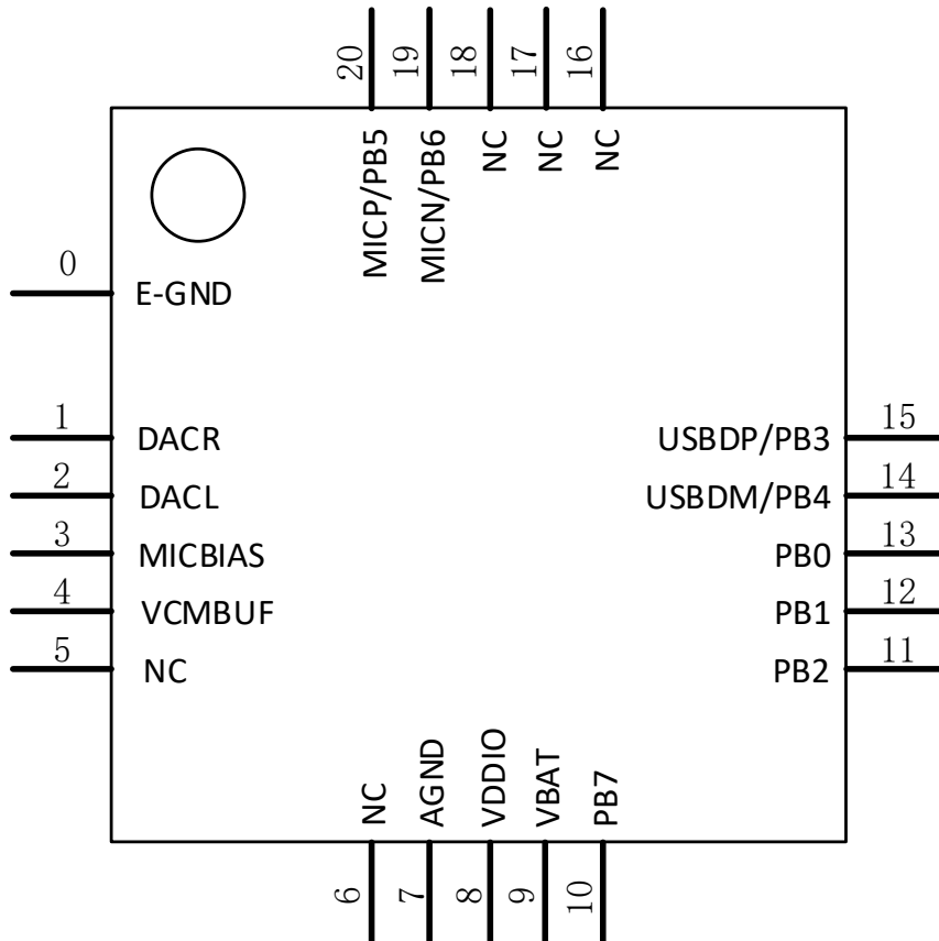
Figure 3-1 Pin Assignment for QFN20
